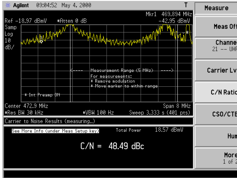
Figure 2-6 Carrier-to-Noise (PAL-B/G)
