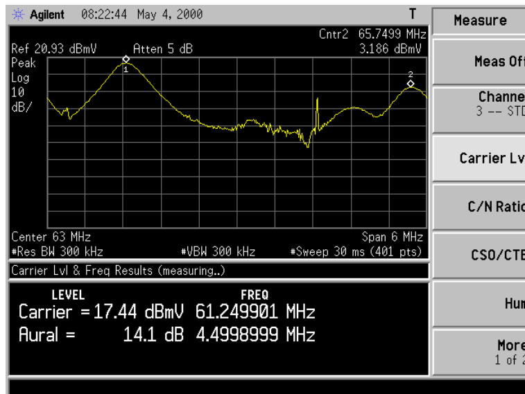
Figure 6-1 Measuring the Visual Level and Aural Carrier Difference (NTSC-M)
