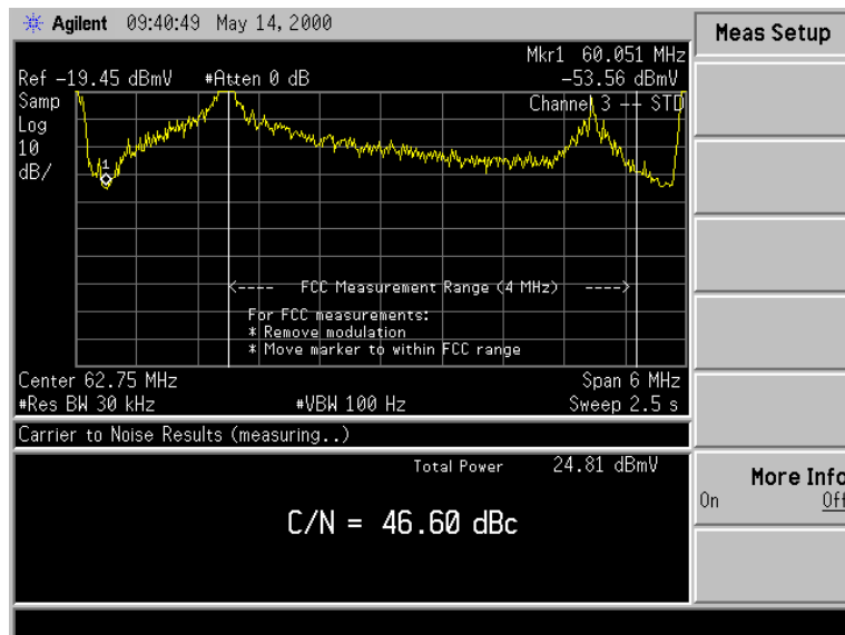
Figure 2-5 Carrier-to-Noise — FCC Measurement Range (NTSC-M)
